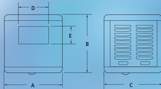
VISTA FRONTAL
